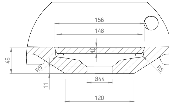
C (1:4)
